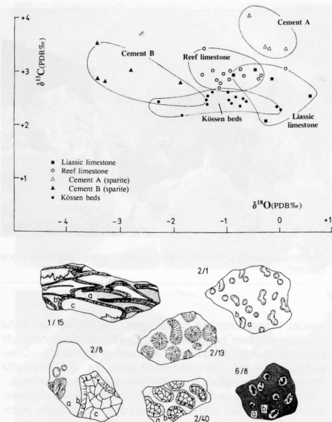
Text-Fig. 3. Cross-plot of \delta^{13}\text{C} and \delta^{18}\text{O} variations in carbonate rocks from the Steinplatte region and some typical samples analysed.
